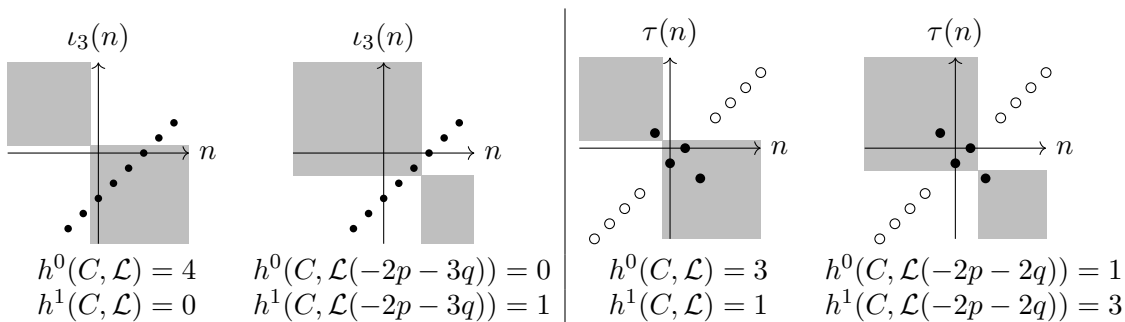
FIGURE 1. Two examples of transmission permutations, and what they say about h^0 and h^1 of twists \mathcal{L}(ap - bq) of \mathcal{L} . See Examples Example 1.3 and 1.4.
