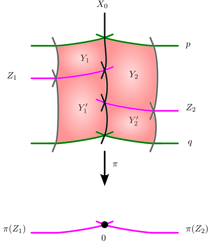
FIGURE 2. A versal deformation of a chain, and the divisors Y_i, Y'_i .
